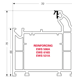
OVOLO LARGE MAIN FRAME - EWS 7706
