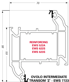
OVOLO INTERMEDIATE TRANSOM 'Z' - EWS 7723
