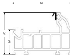
THERMALOGIK FRAME - EWS 7701
